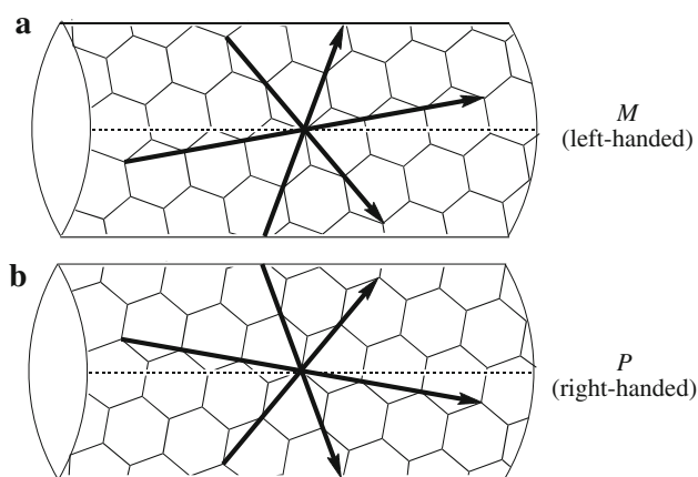
Fig. 7 Definition of M (left-handed) and P (right-handed) of SWNTs. Three arrows and dashed line indicate zigzag lines (Z lines) and SWNT axis, respectively
